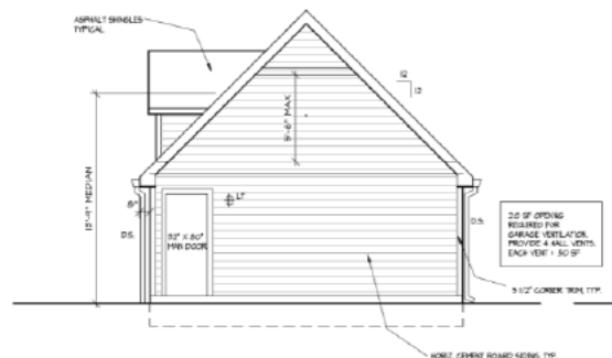
SOUTH SIDE SCALE: 1/4" = 1'-0"
