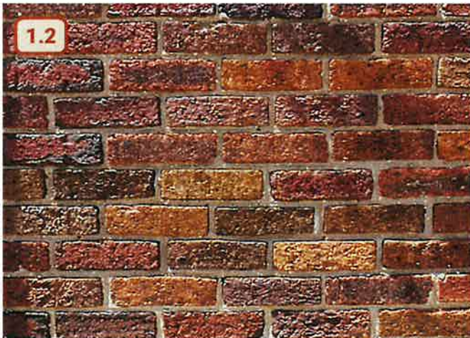
✓ Figure 30. Acceptable tuckpointing
