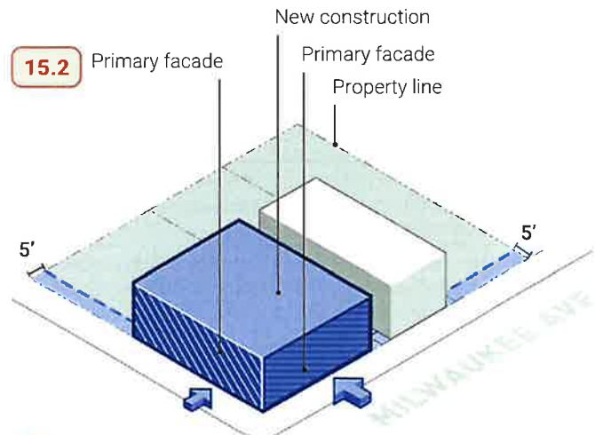
✓ Figure 64. Acceptable setback and orientation at corner-block lots
