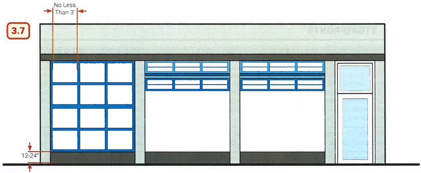
✓ Figure 36. Acceptable operable storefront
